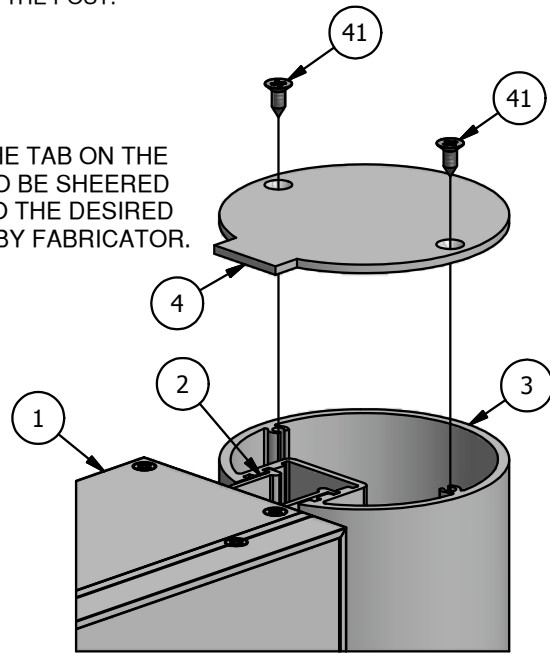
DETAIL B
